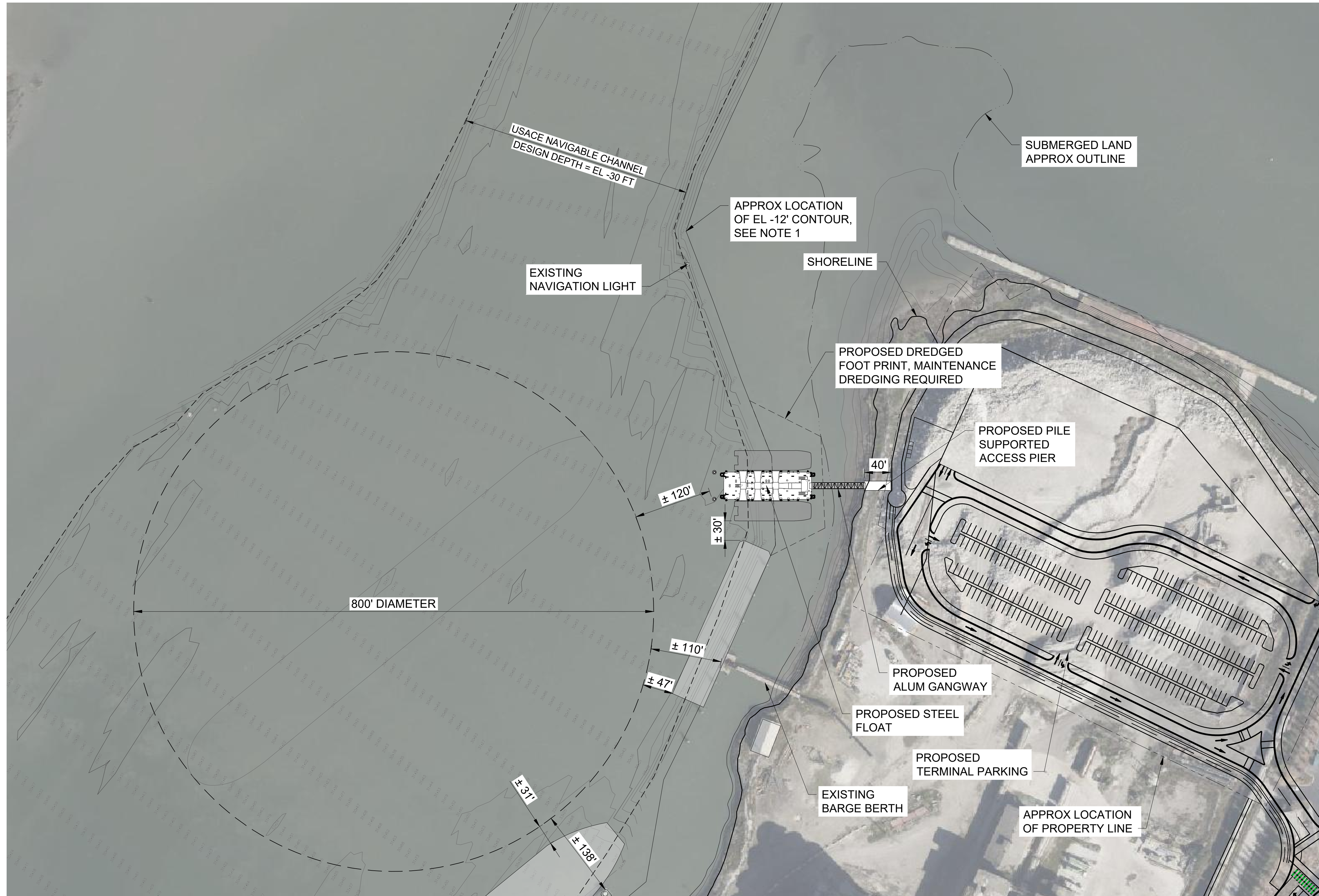
1 FERRY TERMINAL - OPTION C SK-01 SCALE: 1" = 85'-0"
